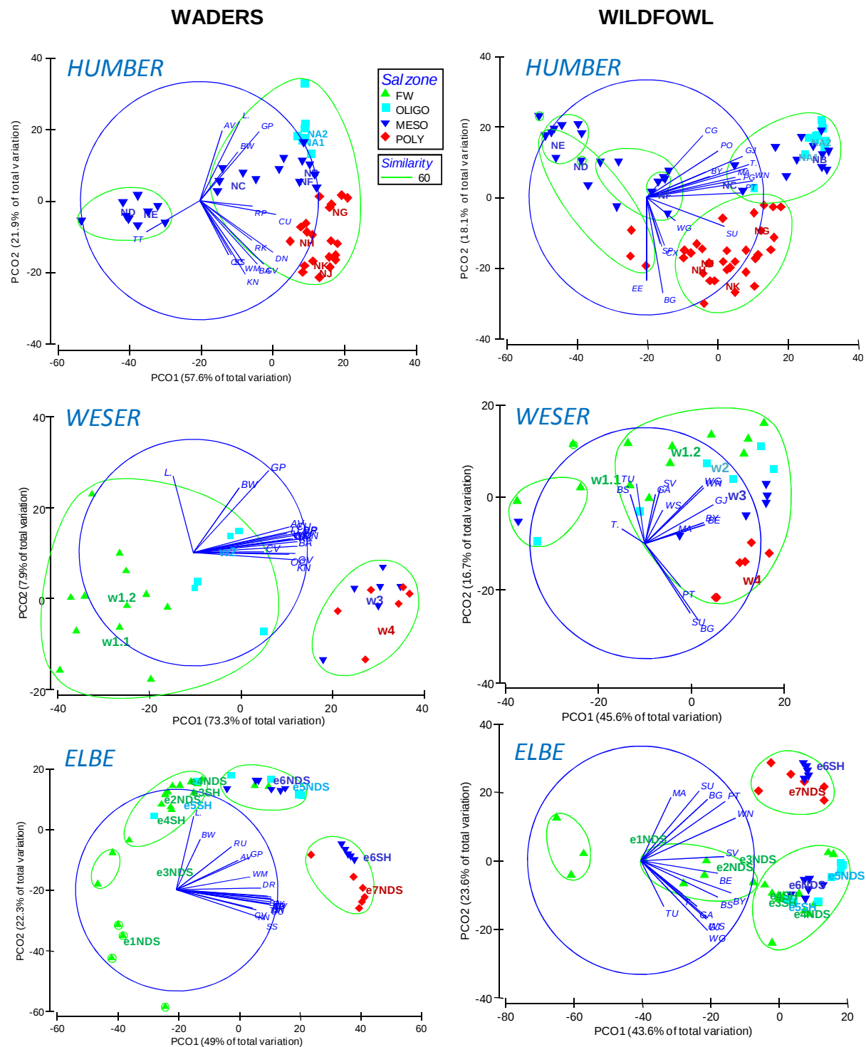
Figure 3.2. Ordination (principal coordinates) analysis of wader and wildfowl assemblages in the Humber, Weser and Elbe estuaries, based on Bray-Curtis similarity calculated on the average species density (ind.km -2 ) by estuarine zone (sectors NA1 to NK in the Humber, zone w1.1 to w4 in the Weser, zone e1 to e7 in the Elbe), period (1=1975-79, 2=1980-84, etc.) and estuarine bank (for Elbe only: NDS=southern bank, SH=northern bank). Vectors indicate the direction of increase in the species density and symbols indicate salinity zones. The centroids of each estuarine zone (with also distinction by estuarine bank in the Elbe) are shown as coloured labels in the graph. Samples showing a similarity in their bird assemblage \geq 60\% (as obtained from cluster analysis – not shown) are grouped by green circles.
