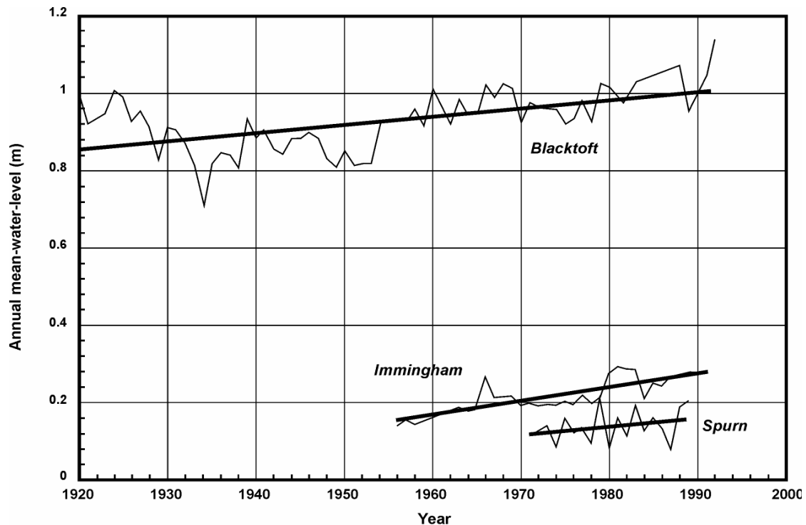
Fig. 2-4: Annual sea-level at 3 locations in the Humber during the 20 th century (Atkins 2002).
