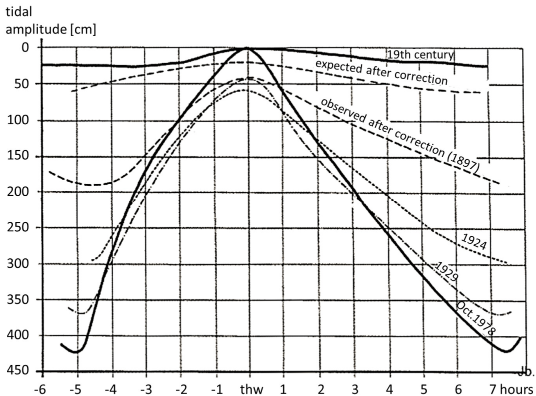
Fig. 2-7: Change of tidal amplitude in the Weser estuary at Bremen City. In the course of deepening projects
