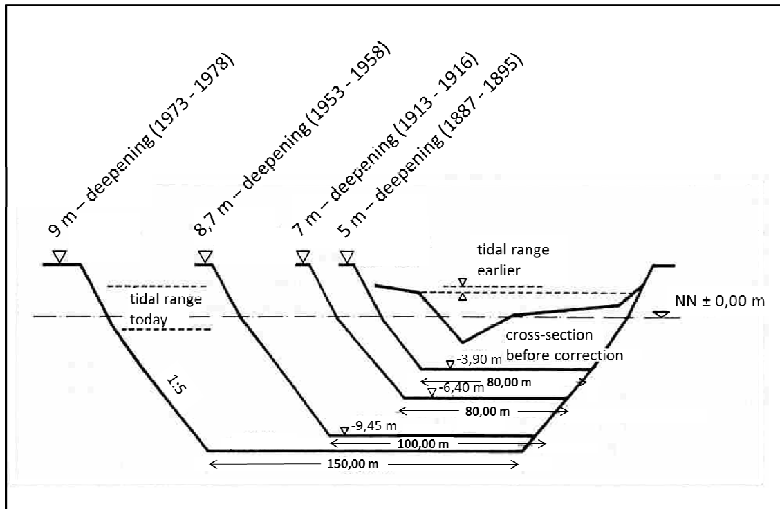
Fig. 2-6: Cross-section of the river bed at Weser km 11 (from Wetzel 1987). Downstream from km 41 a depth of 11,9 m is available and in the Outer Weser the navigational channel provides a depth of 12,5 m; and a further deepening to 13.5 m is planned.
