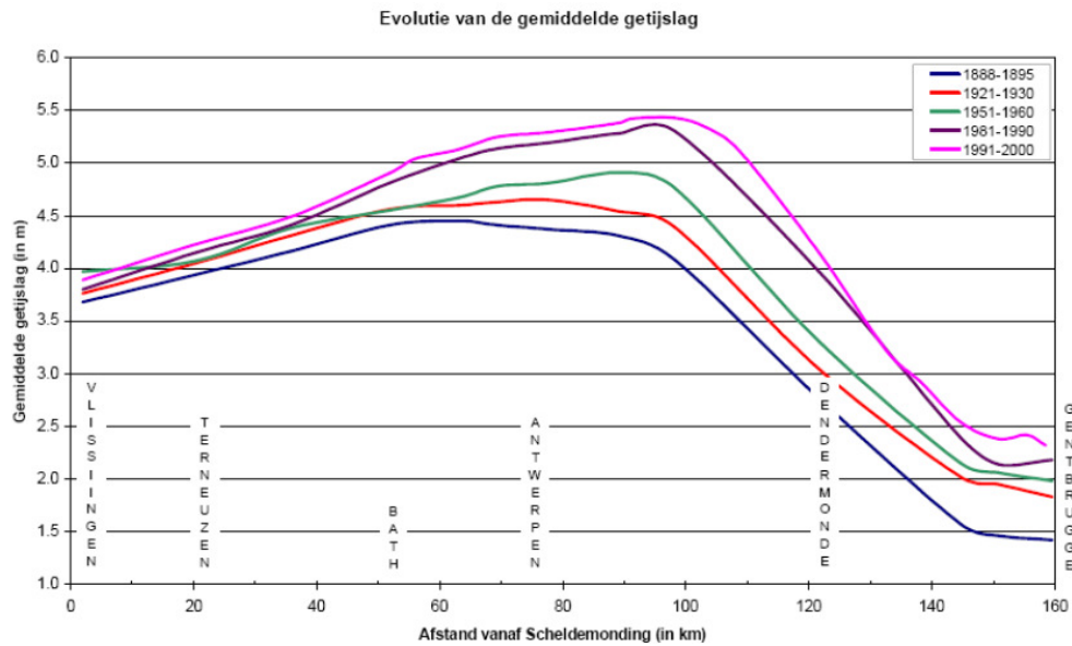
Fig. 2-10: Tidal amplitude along the thalweg of the Scheldt estuary for different times in the 19th and 20th century
